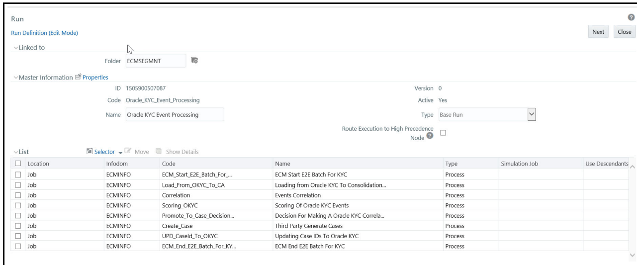
Figure 24. OKYC Connector
